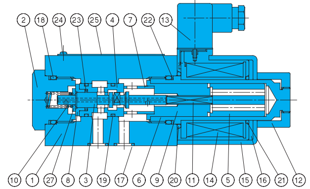
03 SNH-G04-HQ-**-10 06
