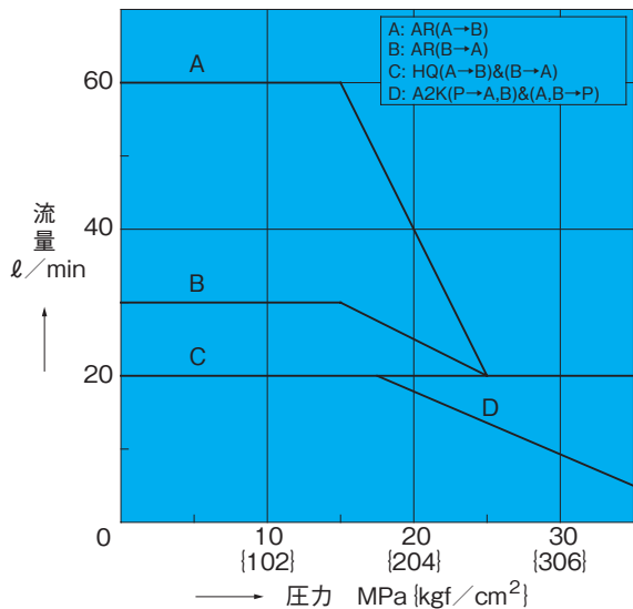
SNH-G04-AR/HQ
