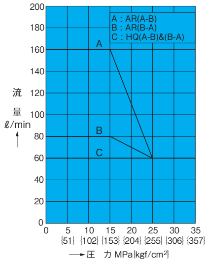
SNH-G04-AR/HQ
