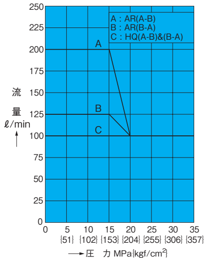
SNH-G06-AR/HQ
