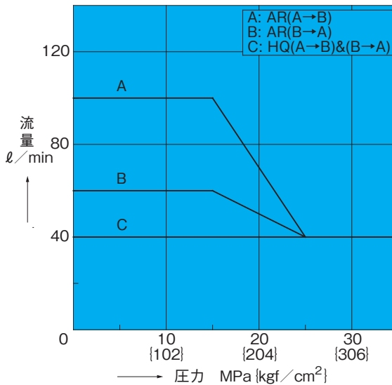
SNH-G06-AR/HQ
